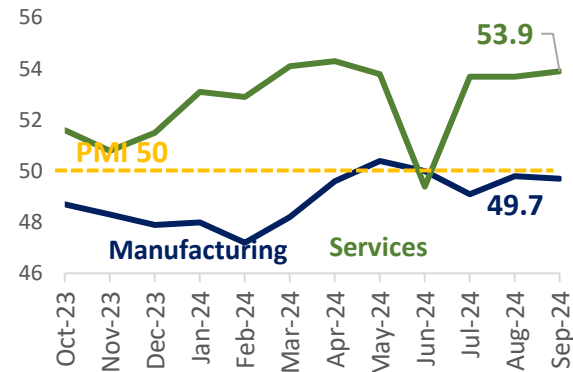
Japan PMI
